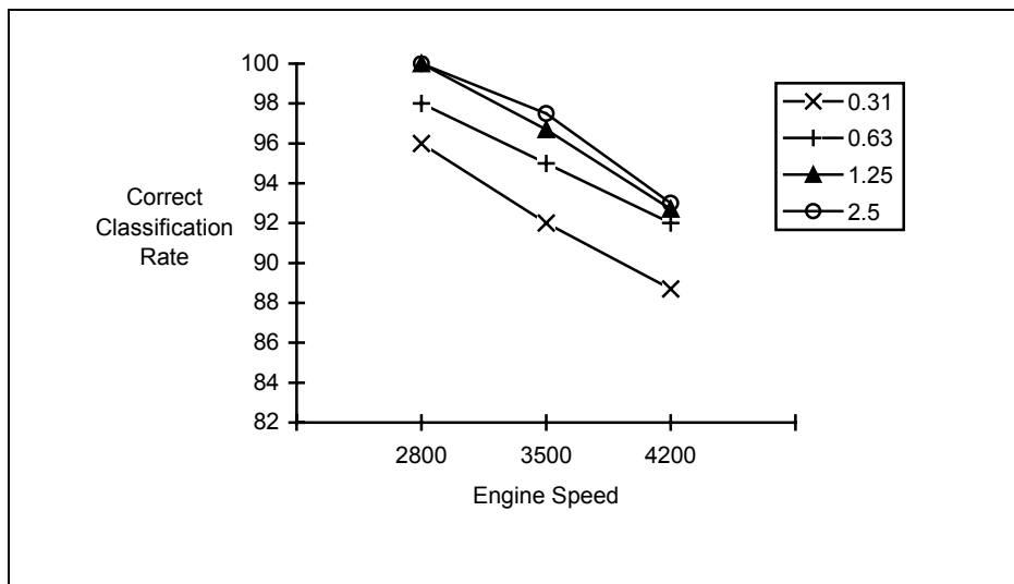
Figure 7: Correct Classification Rate against Engine Speed for Various Normalised Training File Sizes
